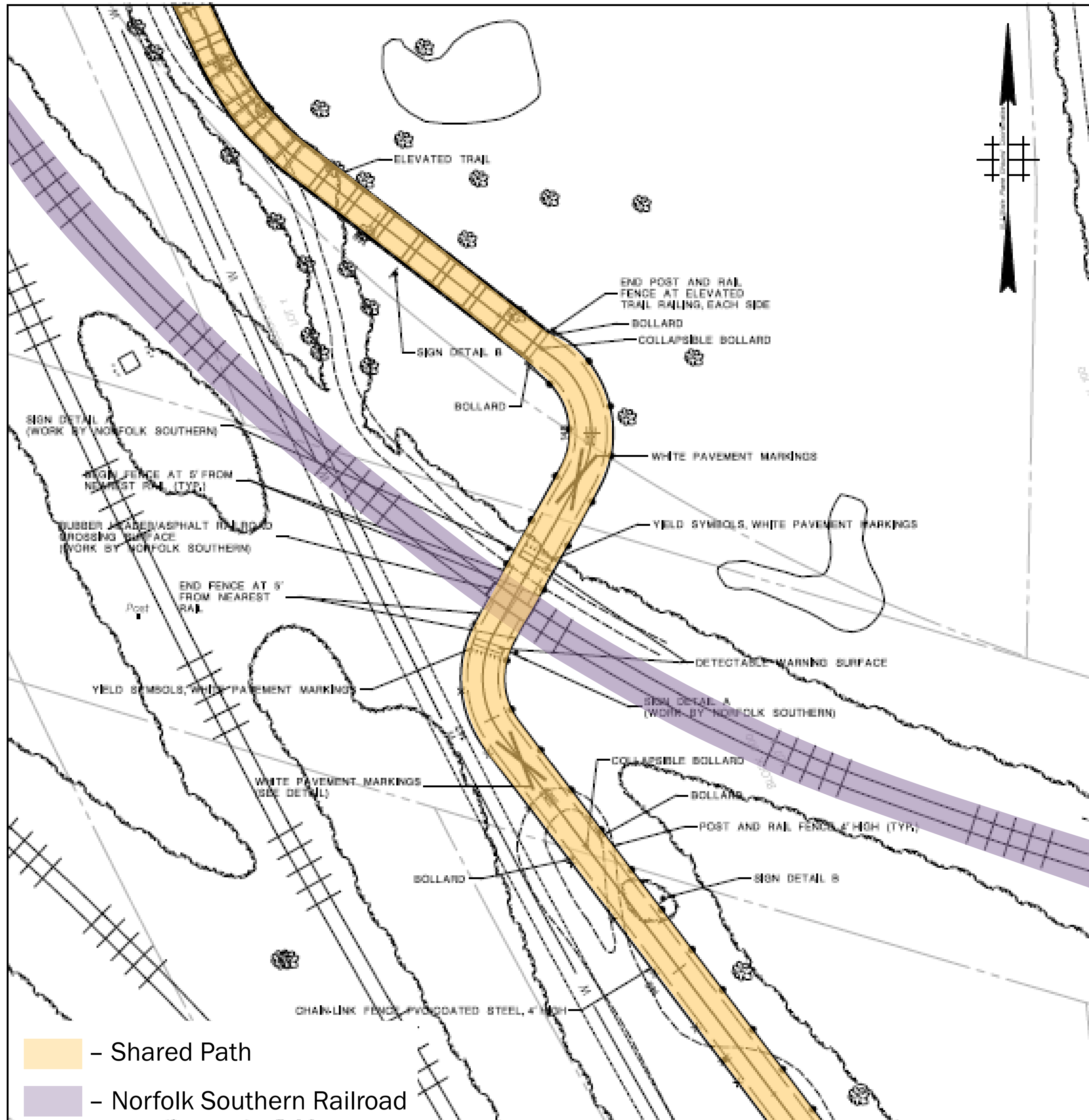
Norfolk Southern Railroad Crossing between Mountain View Boulevard & Meadow Road
