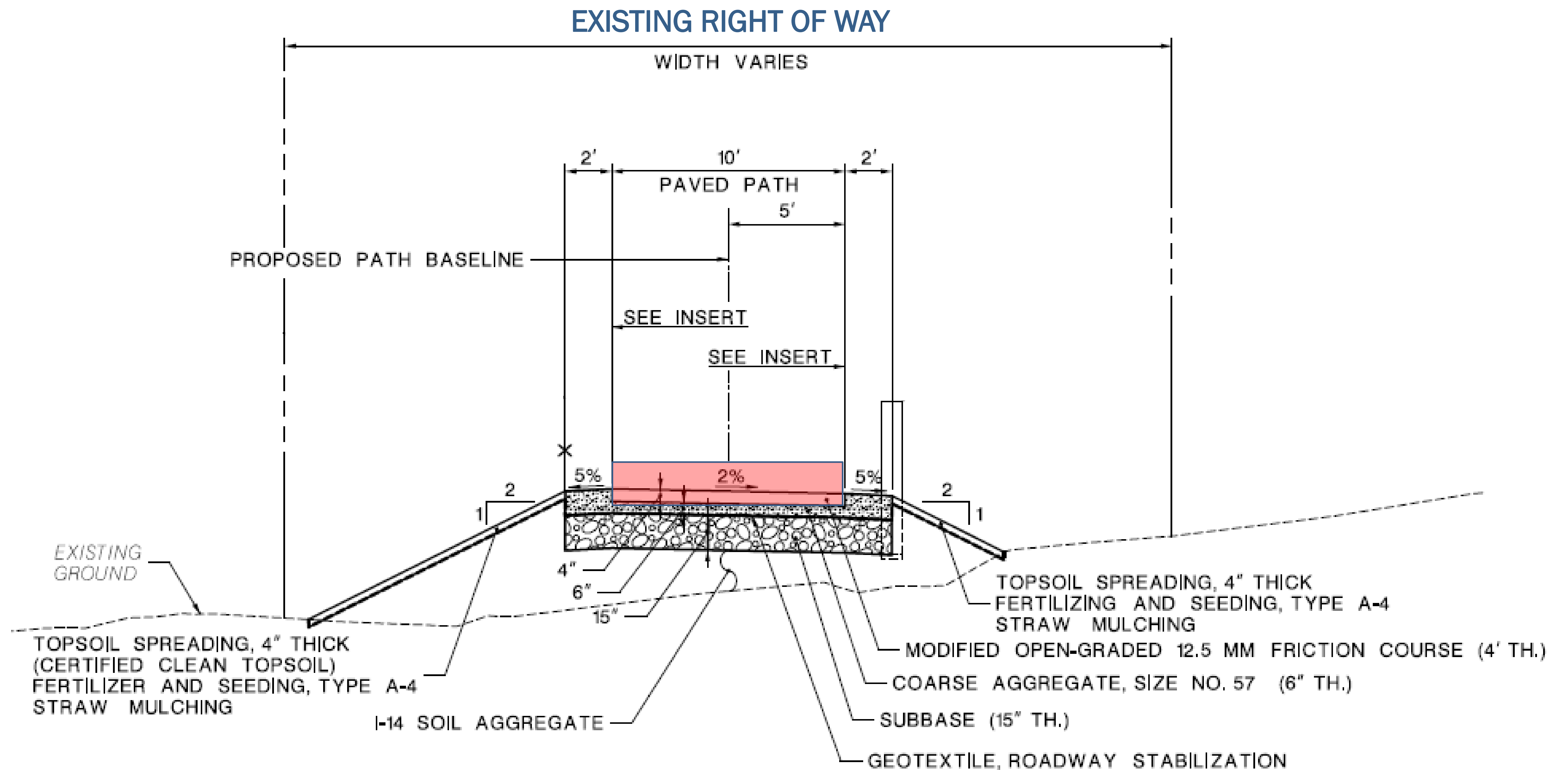
Typical Cross Section View of the Path
