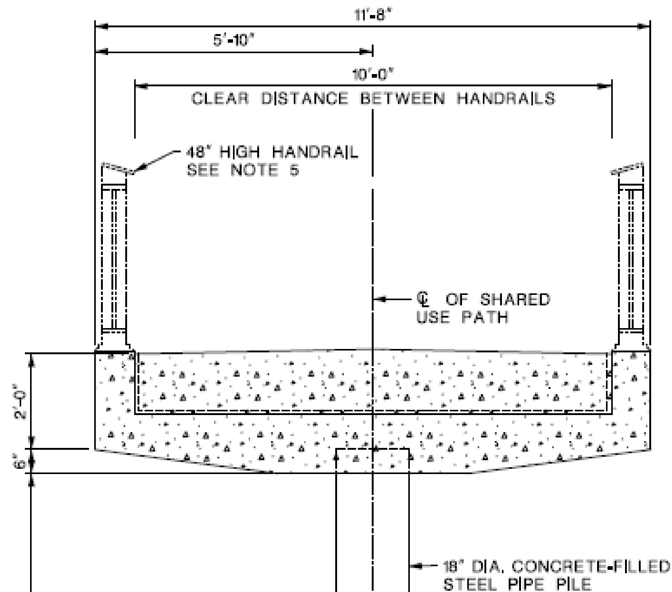
Cross Section View of the Elevated Path
